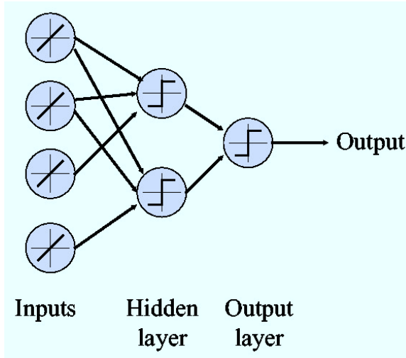
Fig. 5. A schematic diagram of a neural network. Each circle in the hidden and output layer is a computational element known as a neuron
