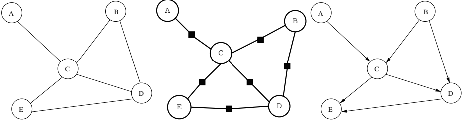
Fig. 1. Three kinds of probabilistic graphical model: undirected graphs, factor graphs and directed graphs
