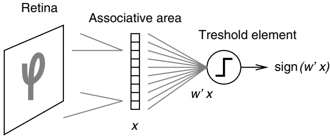
Fig. 3. Rosenblatt’s Perceptron is composed of a fixed preprocessing and of a trainable threshold unit
