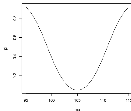
Figure 20.6: Power curve for radon detector.
