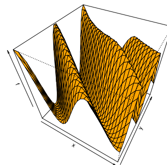
Figure 10.8: Surface plot of function used in Exercise 10.11.
