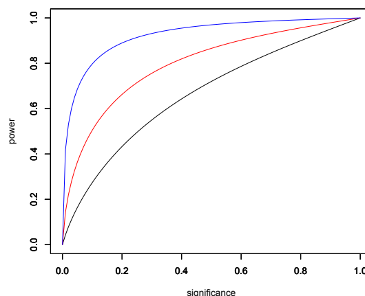
Figure 20.7: Receiver operating characteristic for the radon detector with 6 (black), 12 (red) and 24 (blue) observations and a null \mu_0 = 105 and an alternative \mu = 110 .
