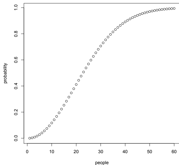
Figure 5.3: The Birthday Problem. For a room of containing k individuals. Using (5.1), a plot of k versus P_k {at least one pair of individuals share a birthday}.
