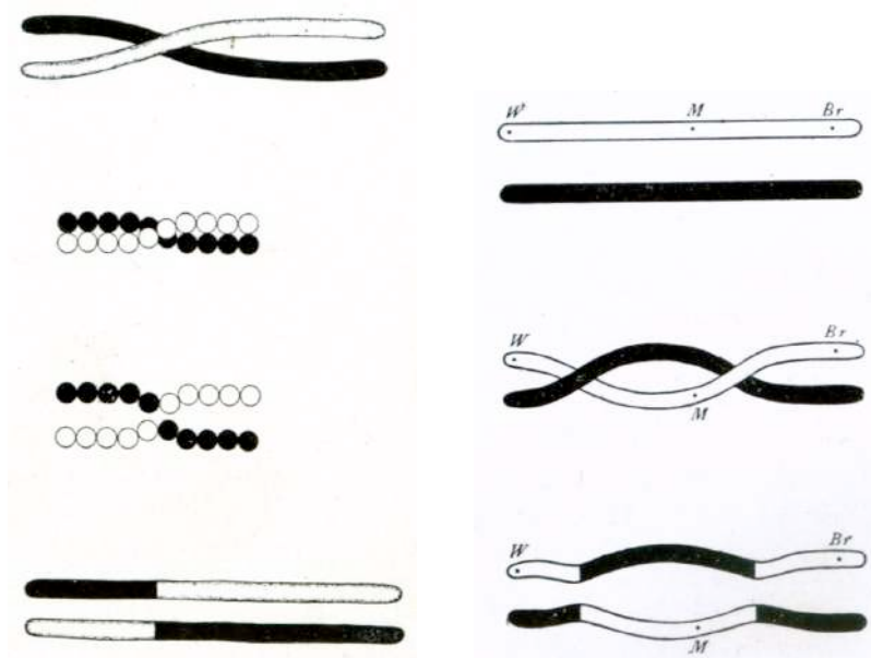
Figure 19.2: Thomas Morgan's 1916 drawings of a (left) single and (right) double crossing over event. The places where homologous non-sister chromatids (newly replicated chromosomes) exchange genetic material during chromosomal crossover during meiosis are called chiasmata (singular: chiasma)
