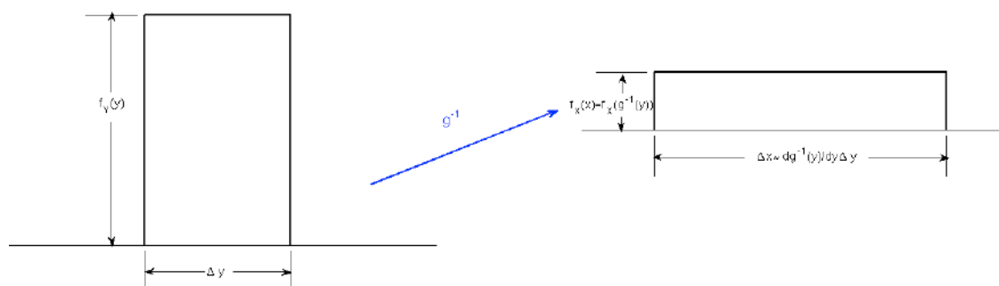
Figure 9.9: Finding the density of Y = g(X) from the density of X . The areas of the two rectangles should be the same. Consequently, f_Y(y)\Delta y \approx f_X(g^{-1}(y)) \frac{d}{dy} g^{-1}(y) \Delta y .
