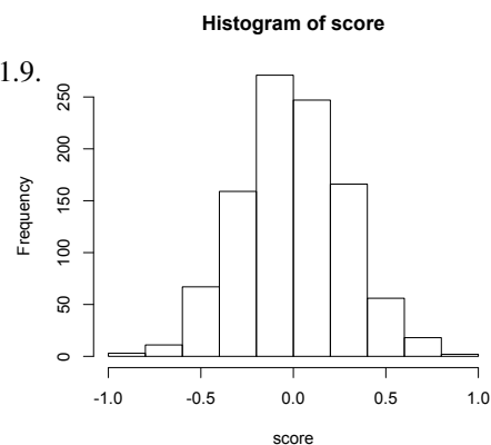
Figure 11.10: 1000 simulations of (S_{2000} - 1000)/\sqrt{2000} , the final values for the simulations above with n = 2000 .
