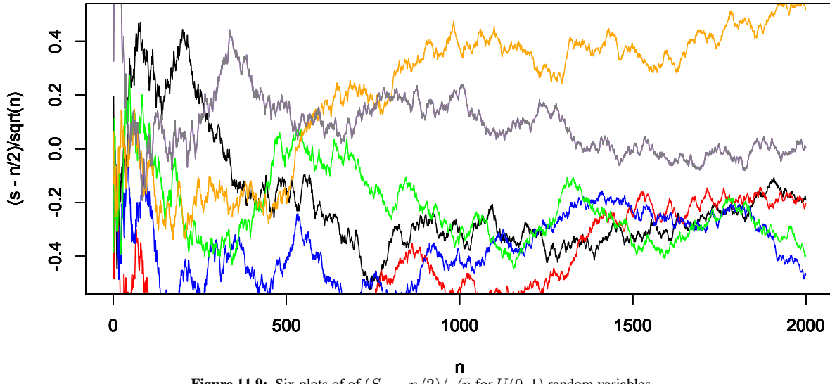
Figure 11.9: Six plots of (S_n - n/2)/\sqrt{n} for U(0, 1) random variables.
