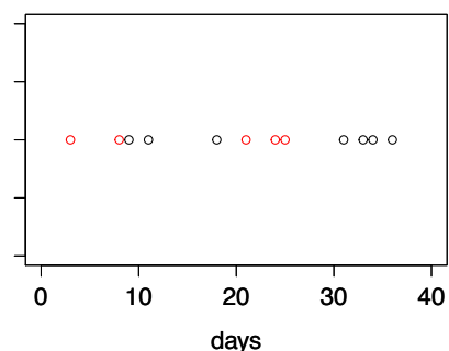
Figure 20.5: Life span in days for 5 transgenic (in red) and 7 wildtype (in black) mosquitoes.
