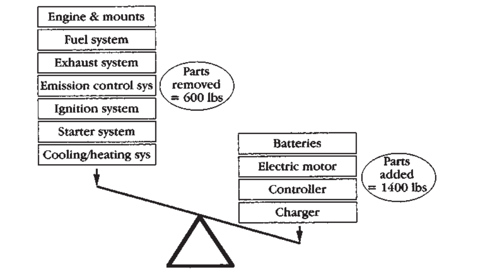
FIGURE 5-3 Front-to-rear weight distribution trade-off.
