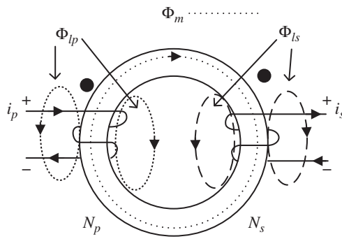
Figure 16.34 Leakage flux.
