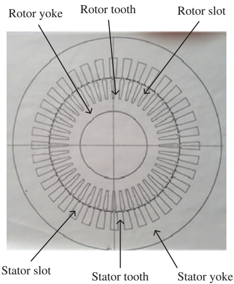
Figure 8.14 Lamination outline for a three-phase four-pole induction machine showing yokes, teeth, and slots of stator and rotor.
