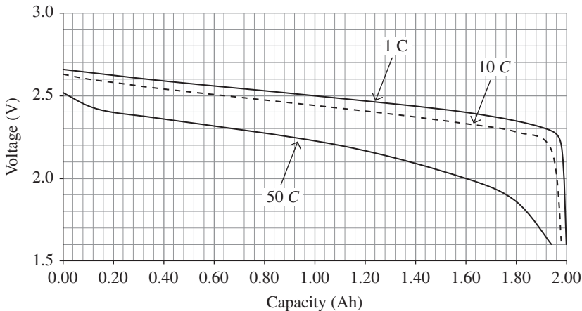
Figure 3.20 Representative discharge curves for a LiT 2.0 Ah battery cell.
