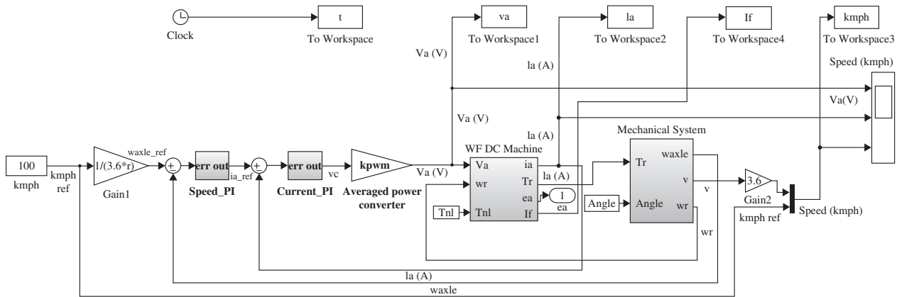
Figure 15.7 Simulink model of WF dc drive.
