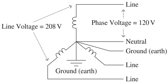
Figure 14.8 Three-phase 208 V system.
