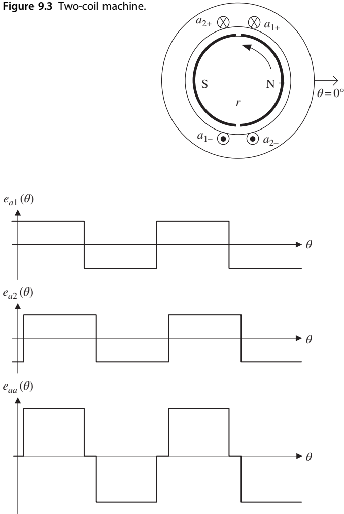
Figure 9.4 Coil and phase voltages for phase a .
