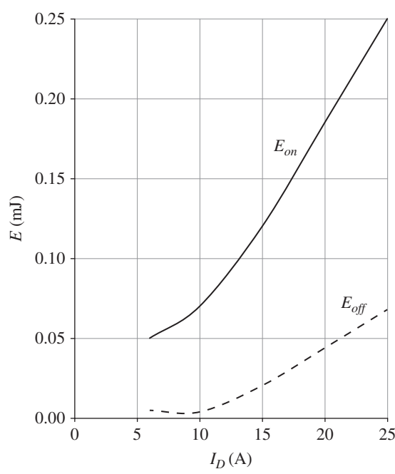
Figure 14.21 Representative 600 V, 15 A MOSFET (and SiC diode) turn-on and turn-off switching losses at 125 ^{\circ}\text{C} and a test voltage of 380 V dc .
