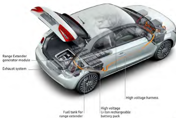
Fig. 14.4 Audi A1 E-Tron concept vehicle with AVL Range Extender in the form of a Wankel Motor. (Source: Audi.)
