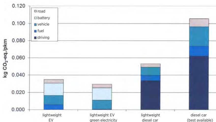
Fig 27.3 Lightweight electric vehicles show the best results in a CO 2 balance. (Source: eco-services 2011.)
