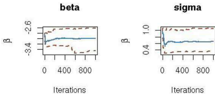
Fig. 8.2. Outcome of the cumuplot function applied to the same MCMC sample as in Figure 8.1. The lower plot corresponds to the lower 2.5% quantile, the central plot to the median, and the upper plot to the .975% quantile.
