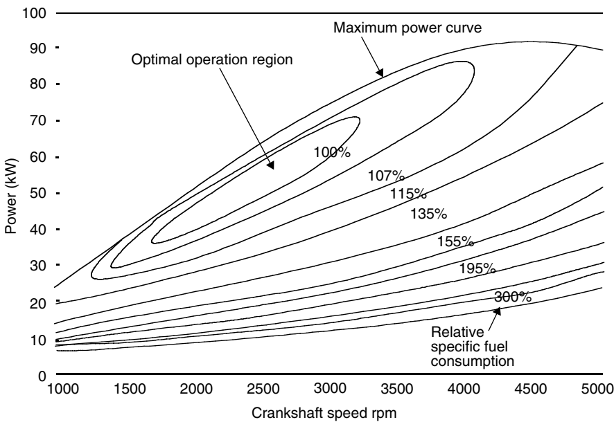
FIGURE 7.2 Example of engine characteristics and optimal operating region
