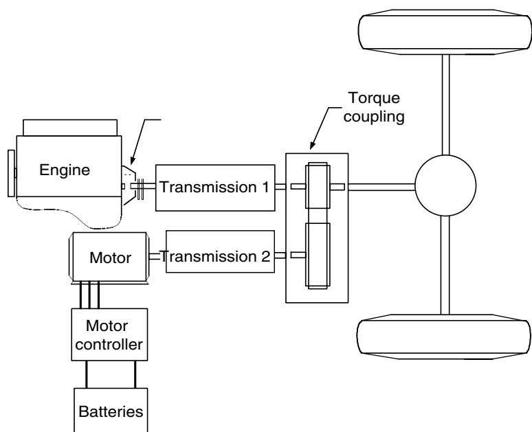
FIGURE 5.8 Two-axle configuration
