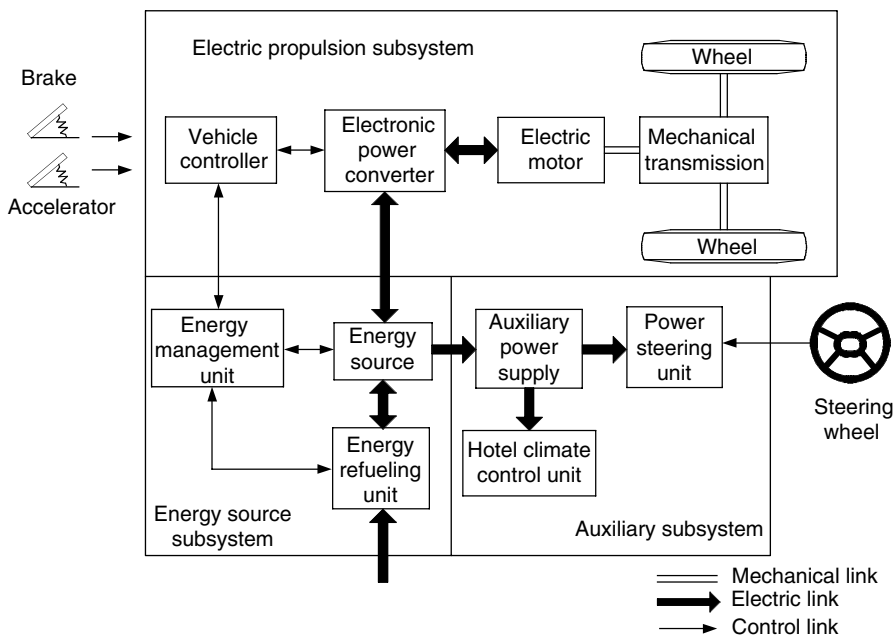
FIGURE 4.2 Conceptual illustration of general EV configuration
