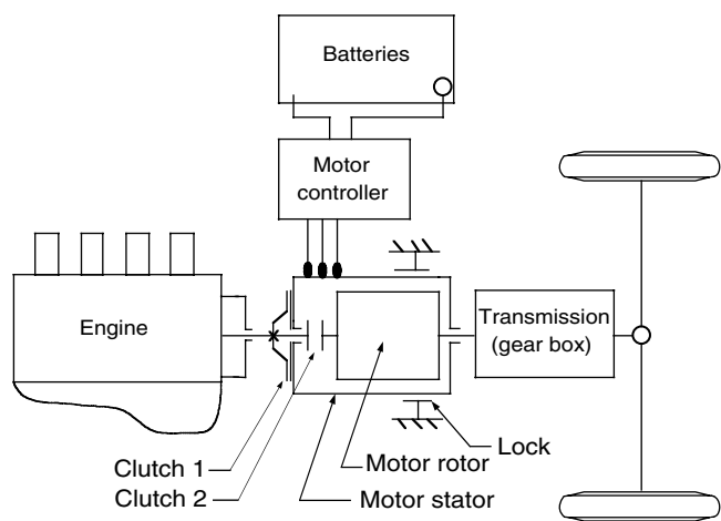
FIGURE 9.18 Series-parallel mild hybrid electric drive train with a floating stator motor
