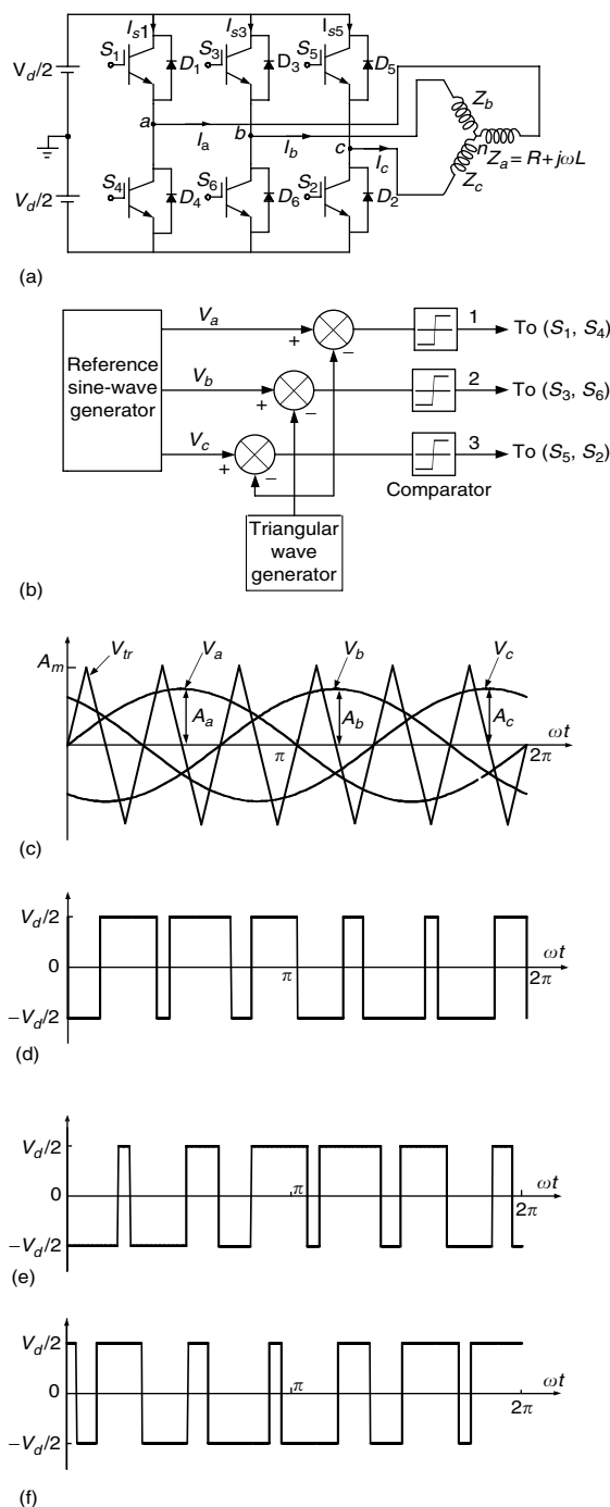
FIGURE 6.21 DC/AC inverter with sinusoidal PWM: (a) inverter topology; (b) control signals; (c) three phase reference voltage and a common isosceles triangular carrier wave; (d) voltage of phase a ; (e) voltage of phase b ; and (f) voltage of phase c
