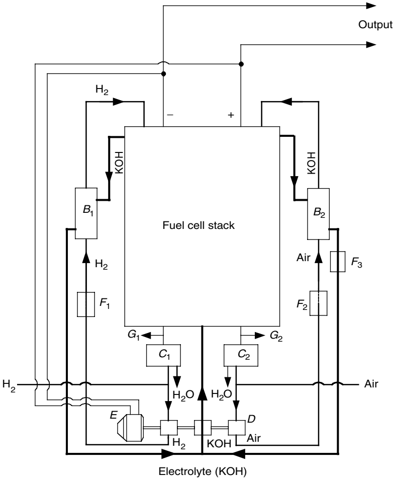
FIGURE 12.7 Circulating electrolyte and supplies of hydrogen and air in an AFC: B_1, B_2 , heater exchangers; C_1, C_2 , condensers; D , pumpers; E , motor; F_1, F_2, F_3 , controls; G_1, G_2 , outlets 1
