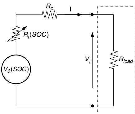
FIGURE 9.8 Battery model
