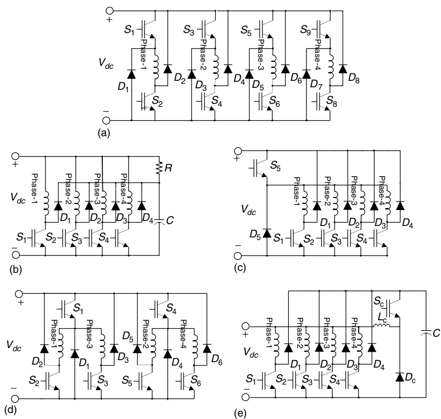
FIGURE 6.62 Different inverter topologies for SRM drives: (a) classical half bridge converter; (b) R-dump; (c) n+1 switch (Miller converter); (d) 1.5n switch converter; and (e) C-dump
