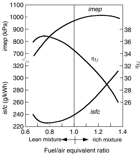
FIGURE 3.8 Fuel/air ratio effect on \text{imep} , fuel conversion efficiency, and \text{isfc}
