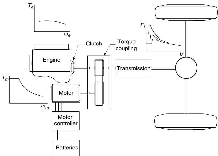
FIGURE 5.10 Two-shaft configuration
