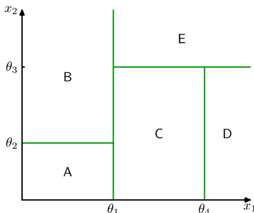
Figure 14.5 Illustration of a two-dimensional input space that has been partitioned into five regions using axis-aligned boundaries.
