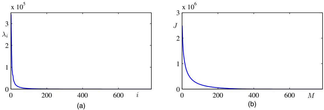
Figure 12.4 (a) Plot of the eigenvalue spectrum for the off-line digits data set. (b) Plot of the sum of the discarded eigenvalues, which represents the sum-of-squares distortion J introduced by projecting the data onto a principal component subspace of dimensionality M .
