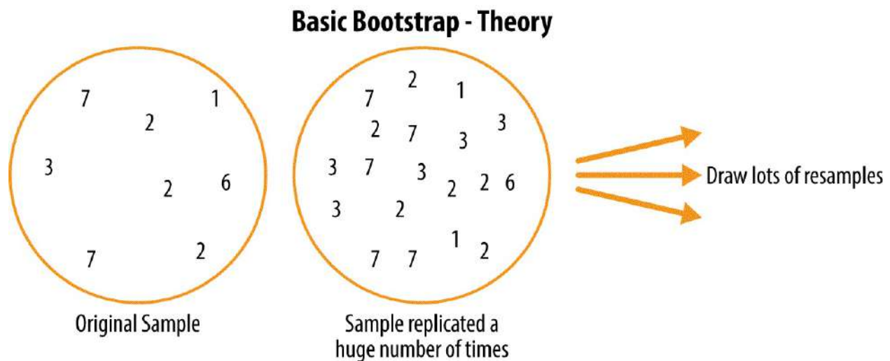
Figure 2-7. The idea of the bootstrap
