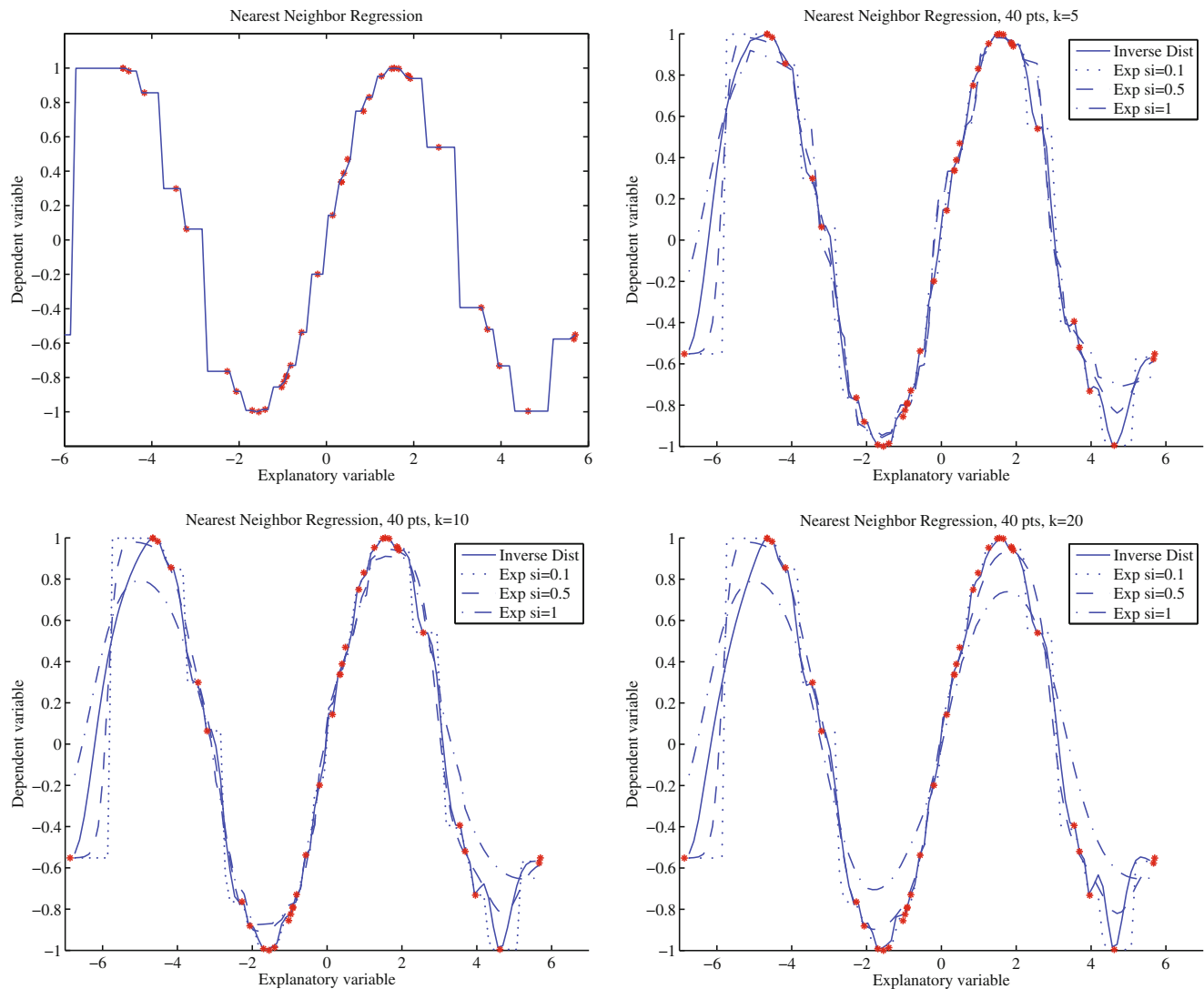
Fig. 13.13 Different forms of nearest neighbors regression, predicting y from a one-dimensional x , using a total of 40 training points. Top left : reporting the nearest neighbor leads to a piecewise constant function. Top right : improvements are available by forming a weighted average of the five nearest neighbors, using inverse distance weighting or exponential weighting with three different scales. Notice if the scale is small, then the regression looks a lot like nearest neighbors, and if it is too large, all the weights in the average are nearly the same (which leads to a piecewise constant structure in the regression). Bottom left and bottom right show that using more neighbors leads to a smoother regression
