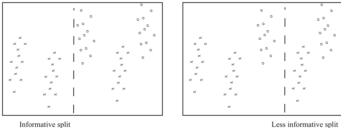
Fig. 11.8 Two possible splits of a pool of training data. Positive data is represented with an 'x', negative data with a 'o'. Notice that if we split this pool with the informative line, all the points on the left are 'x's, and two-thirds of the points on the right are 'o's. This means that knowing which side of the split a point lies would give us a good basis for estimating the label. In the less informative case, about two-thirds of the points on the left are 'x's and about half on the right are 'x's—knowing which side of the split a point lies is much less useful in deciding what the label is
