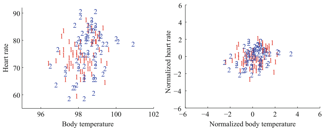
Fig. 2.12 Left : A scatter plot of body temperature against heart rate, from the dataset at http://www2.stetson.edu/~jrasp/data.htm ; normtemp.xls. I have separated the two genders by plotting a different symbol for each (though I don't know which gender is indicated by which letter); if you view this in color, the differences in color makes for a greater separation of the scatter. This picture suggests, but doesn't conclusively establish, that there isn't much dependence between temperature and heart rate, and any dependence between temperature and heart rate isn't affected by gender. The scatter plot of the normalized data, in standard coordinates, on the right supports this view
