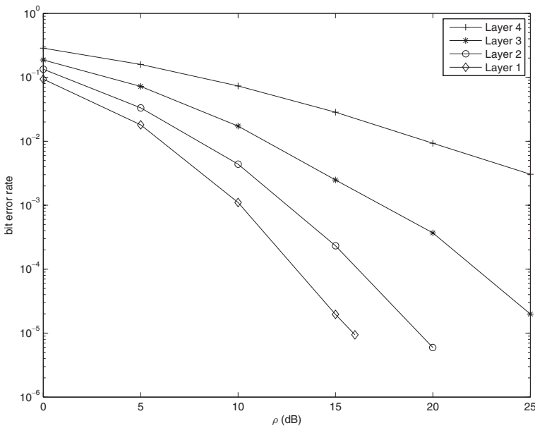
Figure 6.5 VBLAST bit error rate performance for N_t = N_r = 4 for the four layers using the ZF-IC criterion (for uncoded BPSK).
