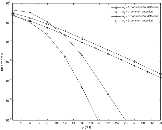
Figure 8.8 Bit error rate performance comparison between the coherent and noncoherent receivers for a USTC with L = 64 and T = 6 for N_r = 1 .
