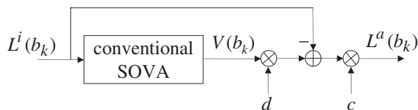
Figure 7.8 Structure of the MSOVA.
