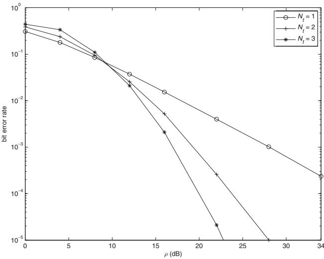
Figure 8.7 Bit error rate performance of a USTC with parameters L = 64 and T = 6 for N_t = 1, 2, 3 and N_r = 1 .
