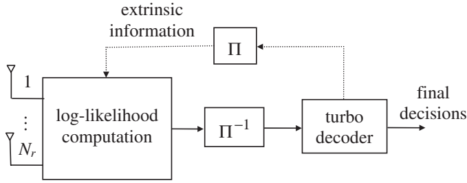
Figure 8.14 Noncoherent iterative TC-USTC decoder.
